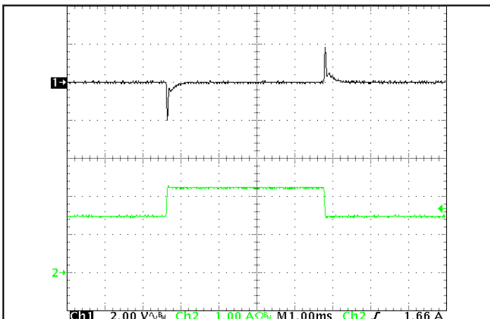
Figure 5: Output voltage response to step-change in load current (50 % -75 % -50 % of I_{out(max)} ; dI/dt = 0.1 A/\mu s ). Load cap: 15 \mu F tantalum cap and 1 \mu F ceramic cap. Ch 1: V_{out} 2 V/div; Ch 2: I_{out} 1 A/div.
