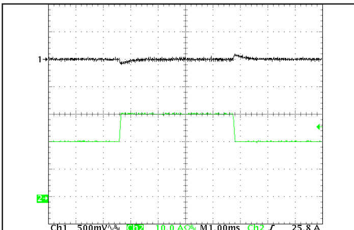
Figure 5: Output voltage response to step-change in load current (50% -75% -50% of I out (max); dI/dt = 0.1 A/μs). Load cap: 15 μF tantalum cap and 1 μF ceramic cap. Ch 1: V out 500 mV/div; Ch 2: I out 10 A/div.
