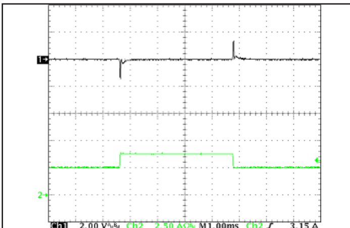
Figure 5: Output voltage response to step-change in load current (50% -75% -50% of I out (max); dI/dt = 0.1 A/μs). Load cap: 15 μF tantalum cap and 1 μF ceramic cap. Ch 1: V out 2 V/div; Ch 2: I out 2.5 A/div.
